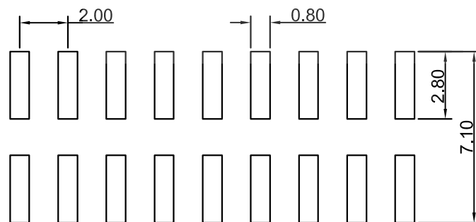
Recommended PCB Board Hole Layout (Tolerance: ±0.05)
